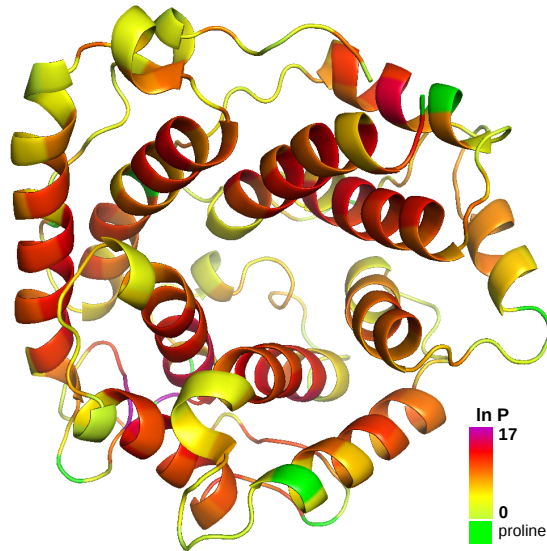
Figure 7 Heat-map visualization of the protection factors of C3d’s residues. Protection factors are derived from, and depicted on, the HDX conformation of C3d. Prolines are coloured in green. Other residues are coloured using a spectrum corresponding to the range of protection values.
