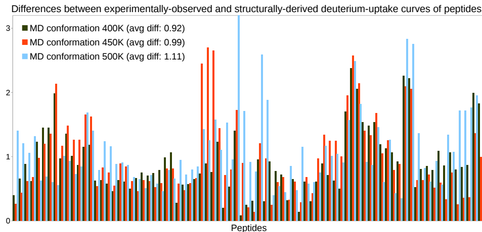
Figure 4 Deriving HDX-MS data from high-temperature MD simulations of C3d. Histograms of differences obtained when assessing the goodness-of-fit between the experimentally-observed HDX-MS data and the HDX-MS data derived from single conformations extracted from MD simulations of C3d at 400 K, 450 K and 500 K respectively.
