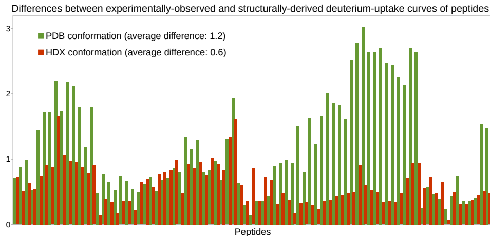
Figure 5 Deriving HDX-MS data from coarse-grained conformational sampling of C3d. Histograms of differences obtained when assessing the goodness-of-fit between the experimentally-observed HDX-MS data of C3d and the HDX-MS data derived from its PDB conformation or its HDX conformation (i.e., the conformation produced by coarse-grained conformational sampling).
