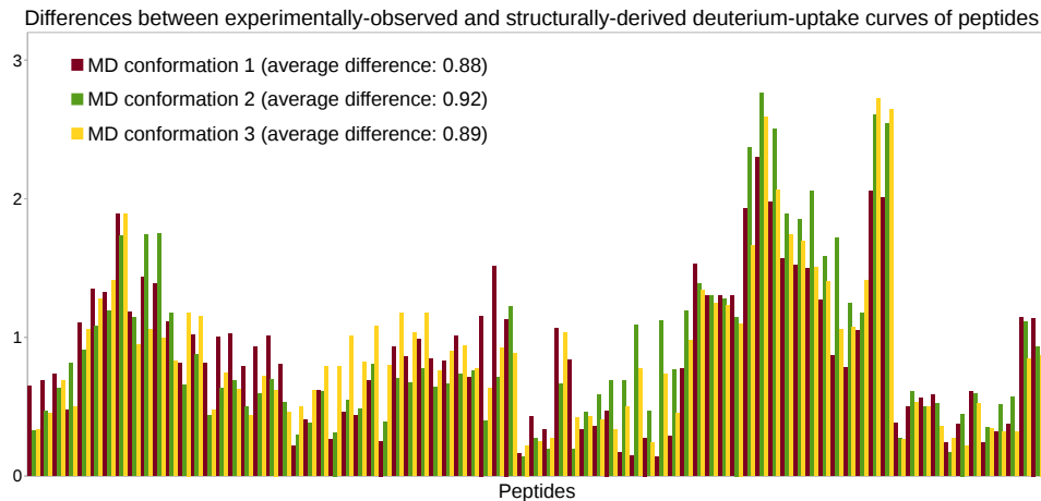
Figure 3 Deriving HDX-MS data from MD conformations of C3d. Histograms of differences (for the 81 peptides of C3d) obtained when assessing the goodness-of-fit between the experimentally-observed HDX-MS data and the HDX-MS data derived from single conformations extracted from three MD simulations of C3d.
