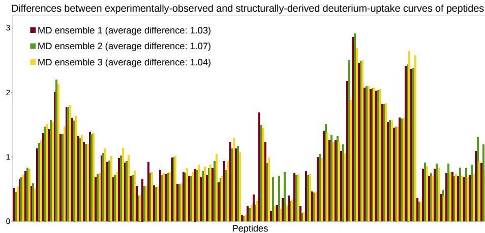
Figure 2 Deriving HDX-MS data from MD simulations of C3d. Histograms of differences (for the 81 peptides extracted from C3d) obtained when assessing the goodness-of-fit between the experimentally-observed HDX-MS data and the HDX-MS data derived from ensembles of conformations extracted from three MD simulations of C3d.
