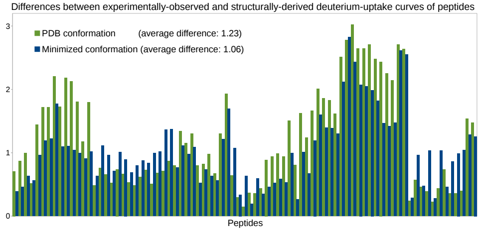
Figure 1 Deriving HDX-MS data from two conformations of C3d. Histograms of differences (for the 81 peptides extracted from C3d) obtained when assessing the goodness-of-fit between the experimental HDX-MS data obtained for C3d and the HDX-MS data derived from the PDB conformation of C3d, or from a minimized version of this conformation.
