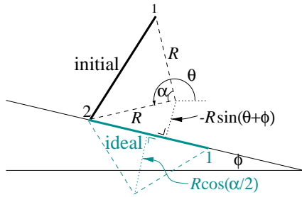
(a) Change in distance between the center of mass and the surface in poses with the initial and ideal orientation
