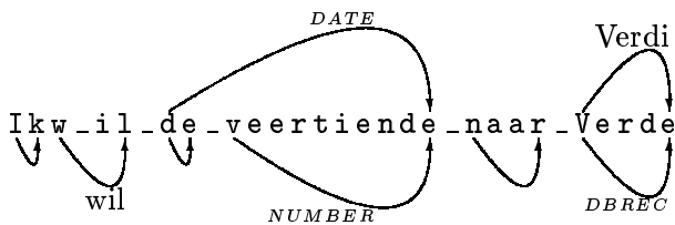
Figure 4: A word graph of an input string
