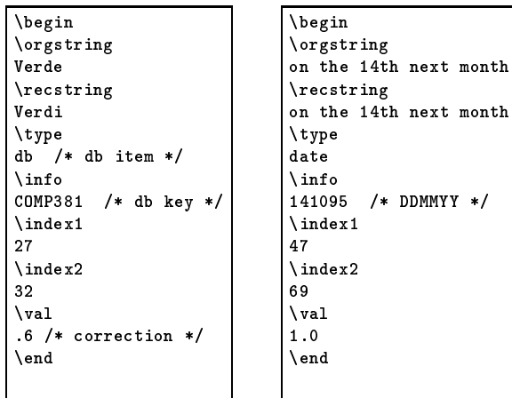
Figure 6: Examples of items output by MAF.
